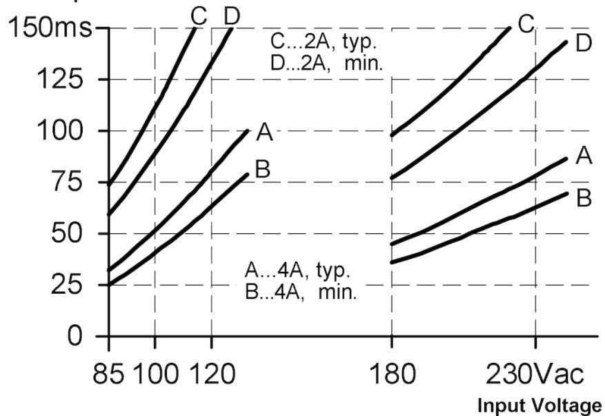
Hold-up Time
