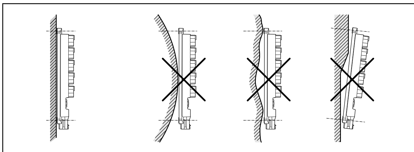
Mounting surface
