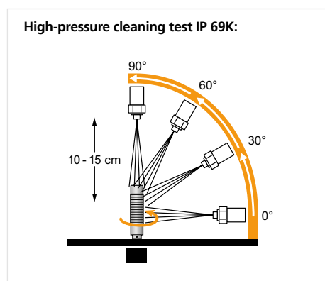
Fine jets of water is sprayed with 100 bar from a distance of 10 to 15 cm. The hot water at 80 °C is sprayed in cycles of 30 seconds.
