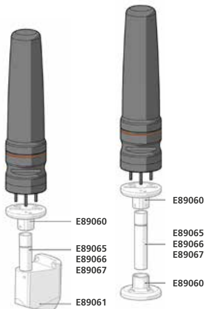
Adapter for side outlet of the cable direct mounting to DV15XX, DV25XX
